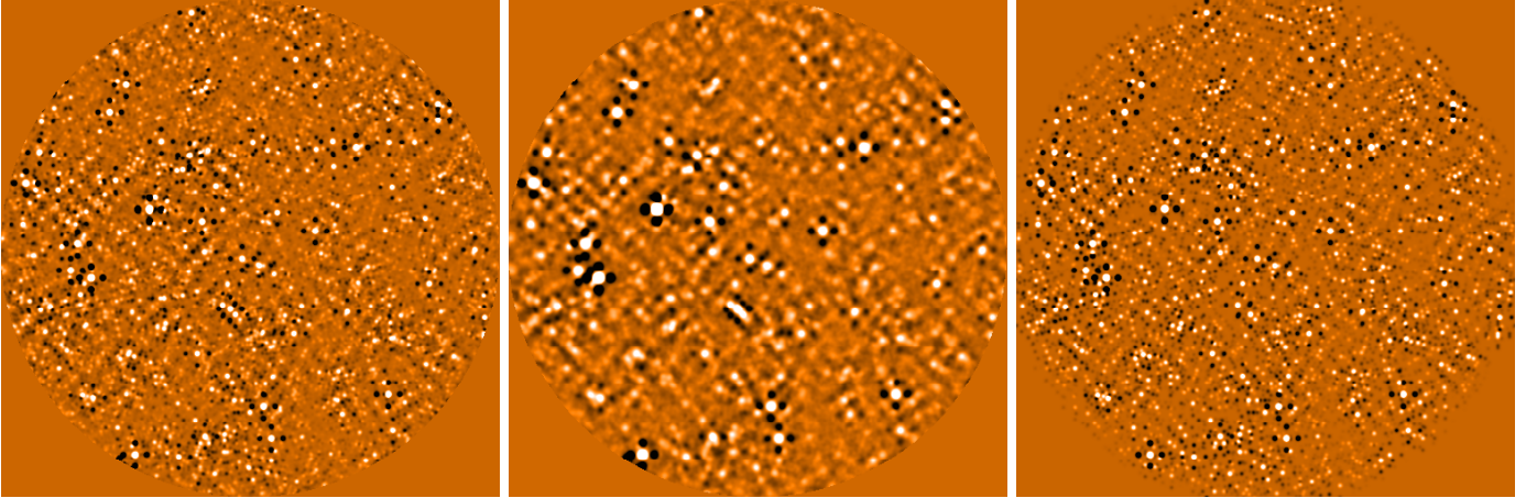
Figure 4: A simulation of the impact of using the deep 450\mu\text{m} survey data to deconvolve the parallel, ultradeep and highly-confused 850\mu\text{m} image ( \sigma_{850} \simeq 0.15\text{mJy} ). The left-hand panel shows a simulated 0.1 sq. degree map, based on current source-count estimates, and including realistic clustering. This is a ‘perfect’ image, with no noise, and convolved to 450\mu\text{m} resolution (FWHM \simeq 8\text{arcsec} ). The middle panel predicts how this patch of sky will actually look, when imaged at 850\mu\text{m} with SCUBA2 on the JCMT, assuming background noise \sigma = 0.15\text{mJy} . The right-hand panel shows the ‘high-resolution’ 850\mu\text{m} image which results from de-convolving the central ‘real’ image with the aid of peak finding algorithms run on the parallel 450\mu\text{m} map (unit scatter in \log(S(450)/S(850)) ), along with \sigma_{450} = 0.5\text{mJy} was assumed when constructing the simulated 450\mu\text{m} map from the left-hand panel). The reclaimed image in the right-hand panel compares well with the input shown on the left, and we find that the number counts at 850\mu\text{m} can be reclaimed to S_{850\mu\text{m}} = 0.6\text{mJy} .
