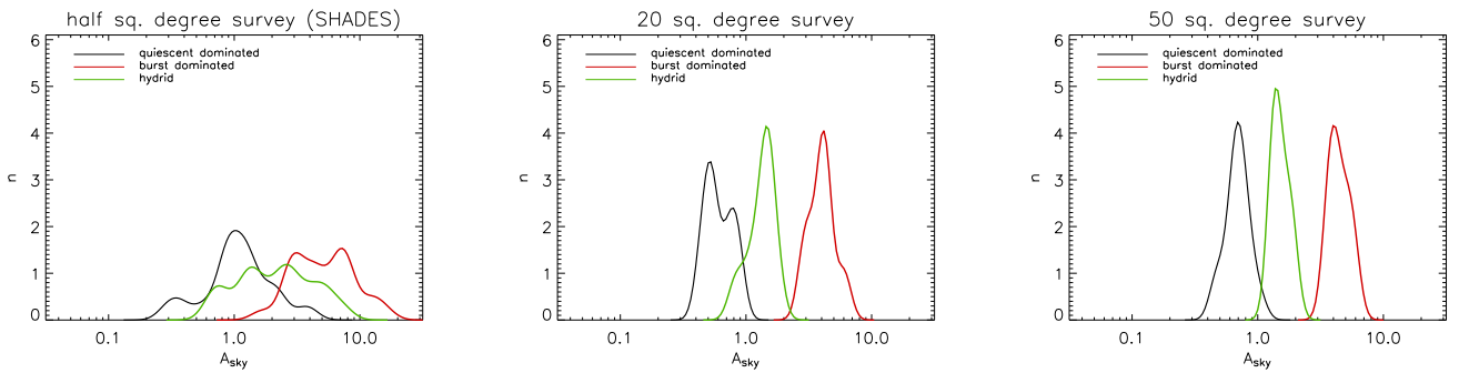
Figure 1: The panels show distributions over predicted clustering amplitudes for the sky-averaged angular correlation function, obtained by fitting this function to 50 mock surveys from a set of simple galaxy-evolution scenarios. The resulting histograms have been smoothed and colour-coded according to the underlying galaxy formation model: the black lines are for a model dominated by quiescent star formation in disks, the red lines represent a starburst-dominated model, whereas the green lines are for a hybrid model in which both star formation modes are important (see van Kampen et al. 2005 for model details). The left-hand panel gives the predictions for the ongoing, 0.5 sq. degree SHADES survey, expected to contain 300 significant sources. The second panel shows the corresponding predictions for the proposed 2-year 20 sq. degree SCUBA2 survey. The diagnostic power of such a survey is clear. The third panel shows the cleanly separated predicted distributions for the 50 sq. degree survey, containing \simeq 20000 sources. For all predictions the effects of noise (at the 0.7 mJy level) and the size of the beam have been included, and the sources have been selected at the 10\text{-}\sigma level (i.e. at 7 mJy).
