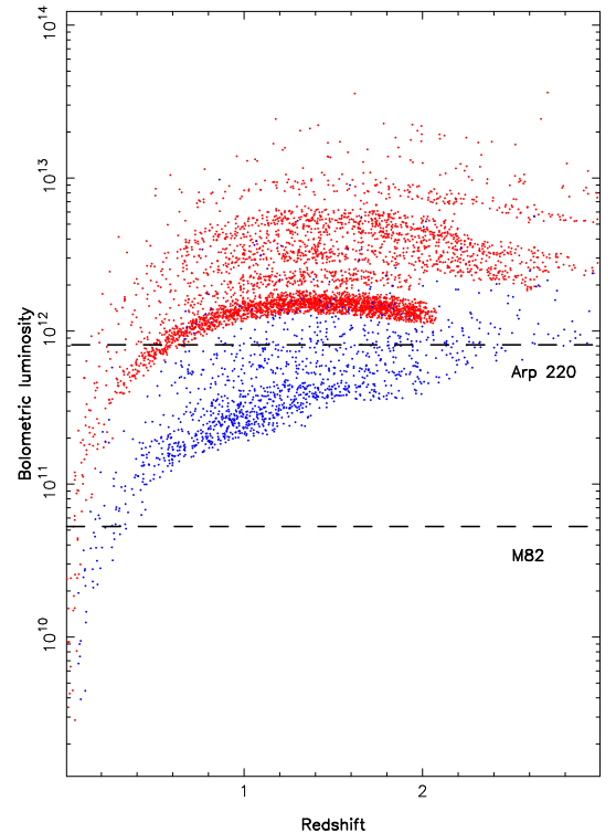
Figure 5: A Monte-Carlo simulation of the coverage of the bolometric luminosity-redshift plane which would be provided by the proposed 2-year survey programme. The simulation adopts a model based on the SCUBA Local Universe and Galaxy Survey (Dunne et al. 2000, MNRAS , 315, 115) and the luminosity-evolution model of Rowan-Robinson (2001, ApJ , 549, 745). The red dots show the sources that will be detected by our 20 sq. degree 850-micron survey; the blue dots the sources that will be detected by the deep 0.6 sq. degree 450-micron survey.
