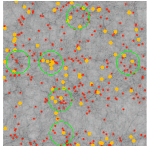
Figure 3: A \Lambda -CDM model at z = 2 with possible sub-mm galaxies highlighted (red < 8 \text{ mJy} , gold > 8 \text{ mJy} ) based on the standard GALFORM prescription for identifying sub-mm sources (Baugh et al. 2005, MNRAS, 356, 1191). The field is 200 Mpc on a side at z = 2 , corresponding to a total area of 42 sq. degrees on the sky. There are 65 > 8 \text{ mJy} sources in this thin redshift (20 Mpc thick) slice, from a total population of \sim 10^4 integrated along the line of sight. The green circles illustrate the radius of a sphere that contains a mass 7 \times 10^{14} M_\odot (Coma-like) before collapse, \sim 16 \text{ Mpc} or 1 degree diameter on the sky. This should serve as a boundary for any material ending up in a present day cluster of this mass.
