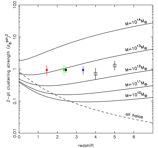
Figure 2: The evolution of the amplitude of the 2-pt statistics – the correlation function and the power spectrum, parameterized by the mean square fluctuations in spheres of radius 8 h^{-1} Mpc. The clustering amplitude for halos of different mass in a concordance \Lambda CDM cosmology (solid lines), and the total matter (dashed line) are compared with the observed clustering strength of the LBGs of Ouchi et al. (2001, ApJ, 558, L83) (open squares) and the expected clustering amplitudes and errors provided by the proposed SCUBA-2 survey (solid symbols – see text for details).
